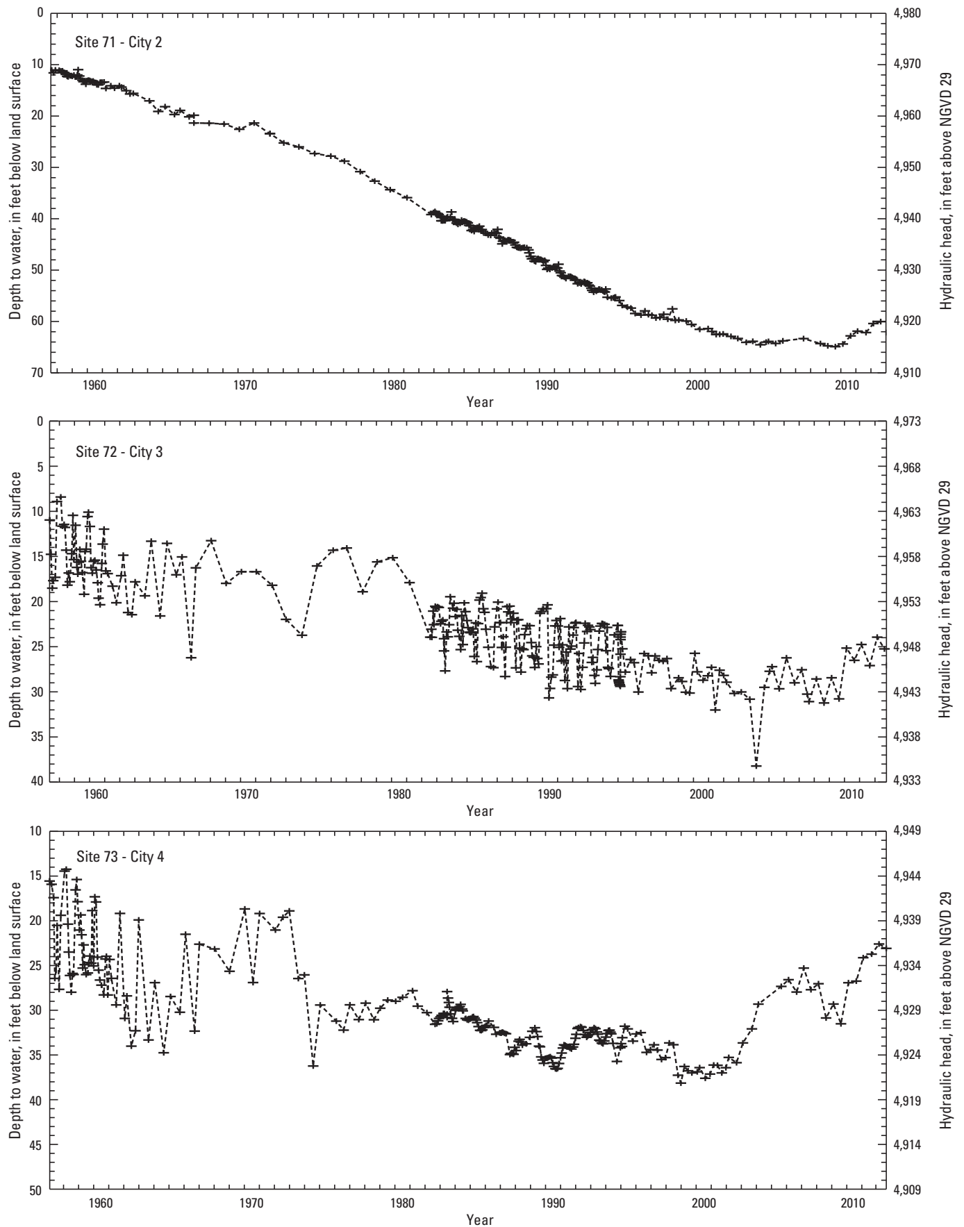
Figure 4. Water-level data for selected wells and piezometers in the Albuquerque Basin, central New Mexico.—Continued
