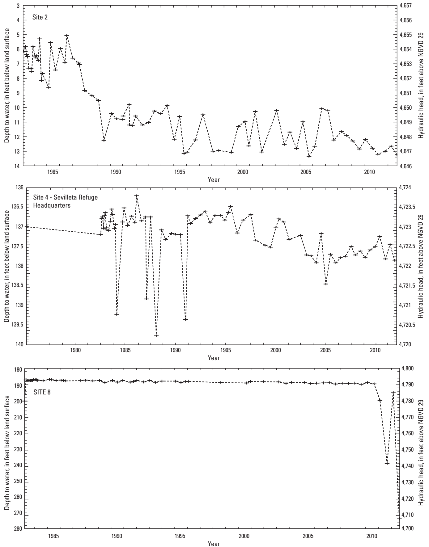
Figure 4. Water-level data for selected wells and piezometers in the Albuquerque Basin, central New Mexico.
