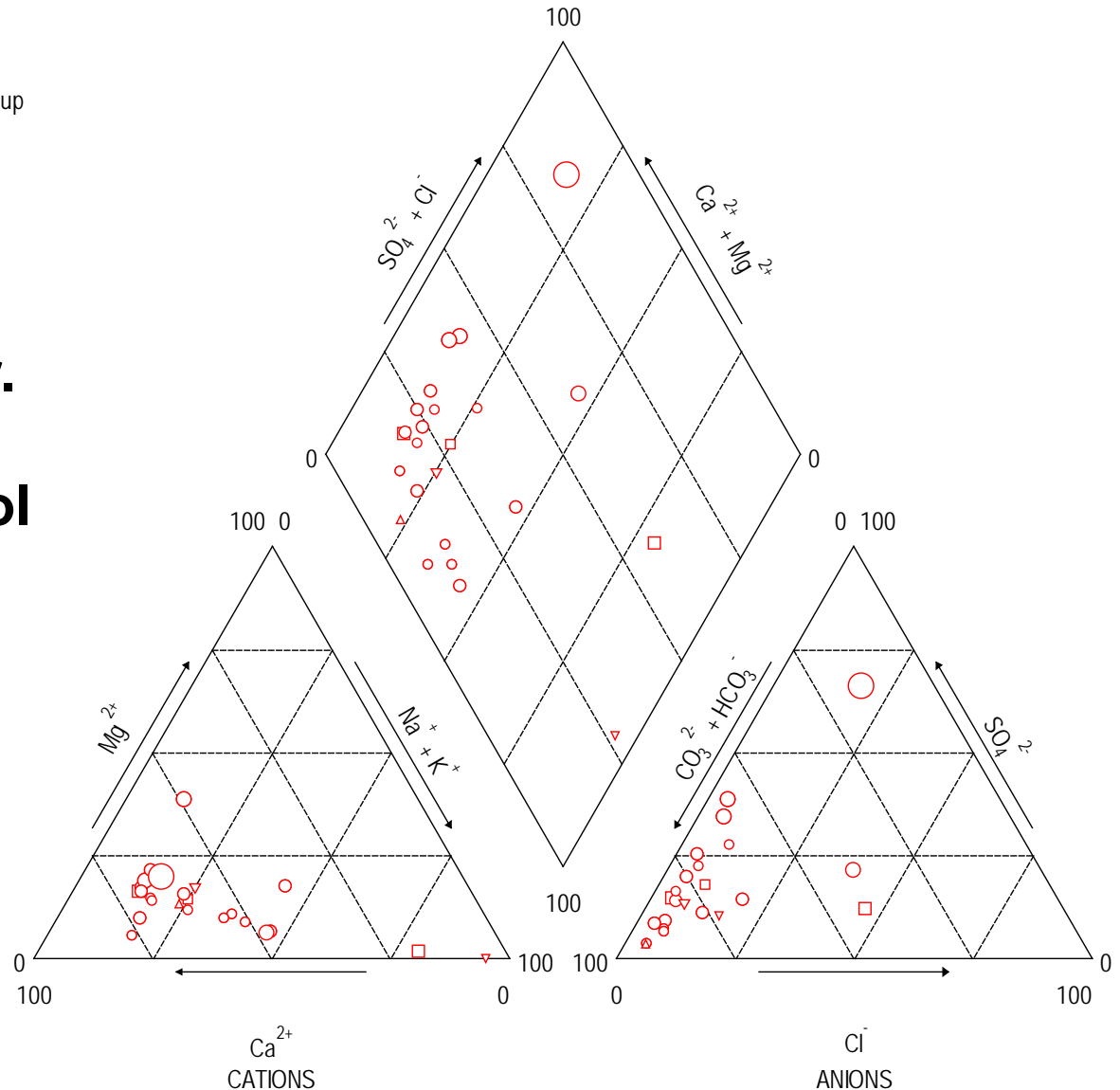
Alamosa Canyon Major Ion Chemistry
