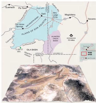
What NIMBARI researchers think the San Agustín Plains would look like from the south without basin-fill. Dark tans show bedrock topography beneath the basin-fill. The proposed development is along western edge of North Basin. Distance from the Very Large Array to Datil is 14 miles.
